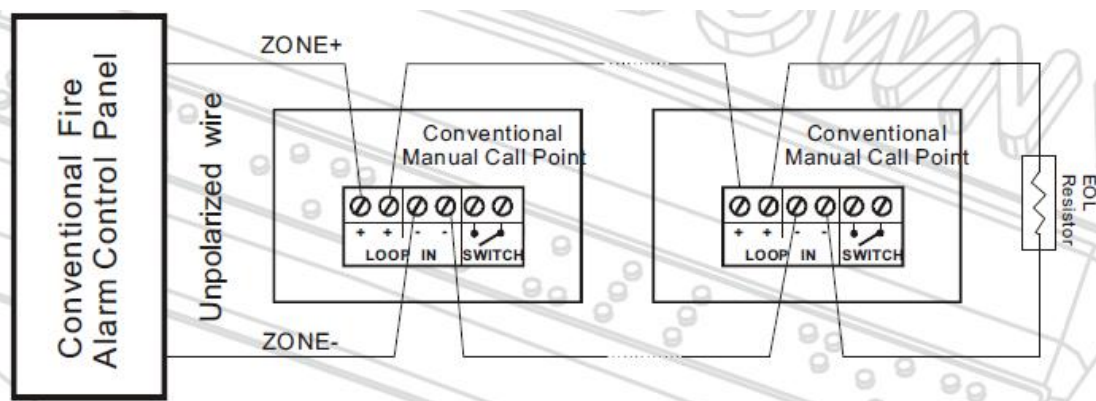
Figure 2. Wiring diagram for the manual call point:
